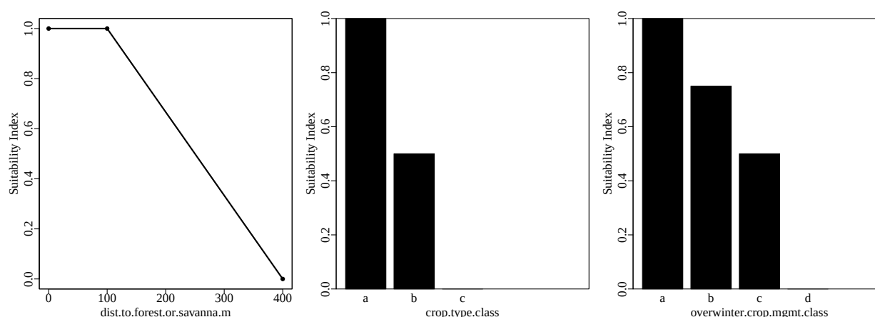
Figure 1. Suitability index graphs for variables included in the easternwildturkeyCroplandShrub model in ecorest .
